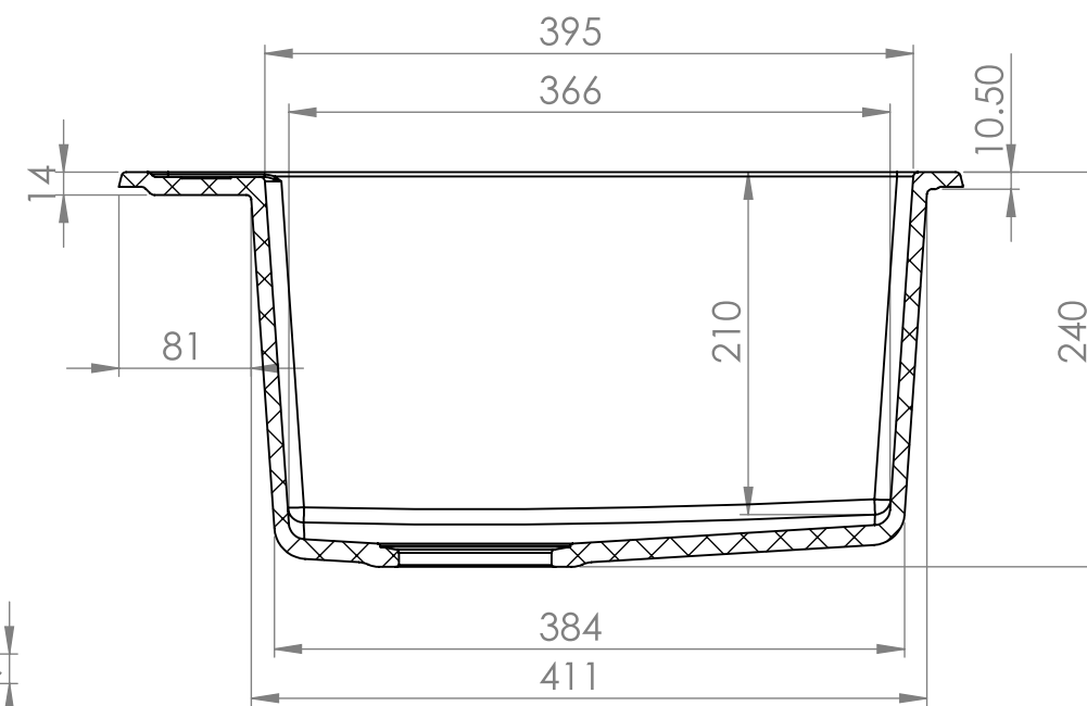
SECTION B-B
