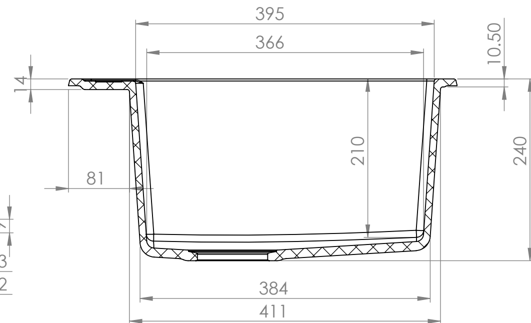
SECTION B-B
