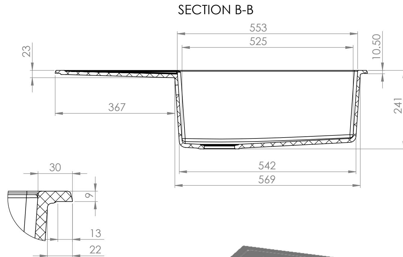
DETAIL C SCALE 1 : 2
