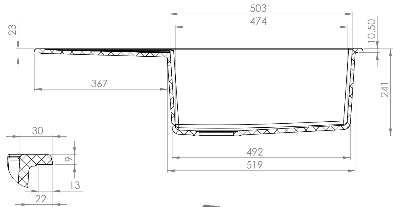
DETAIL C SCALE 1 : 2
