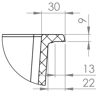
DETAIL D SCALE 1 : 3
