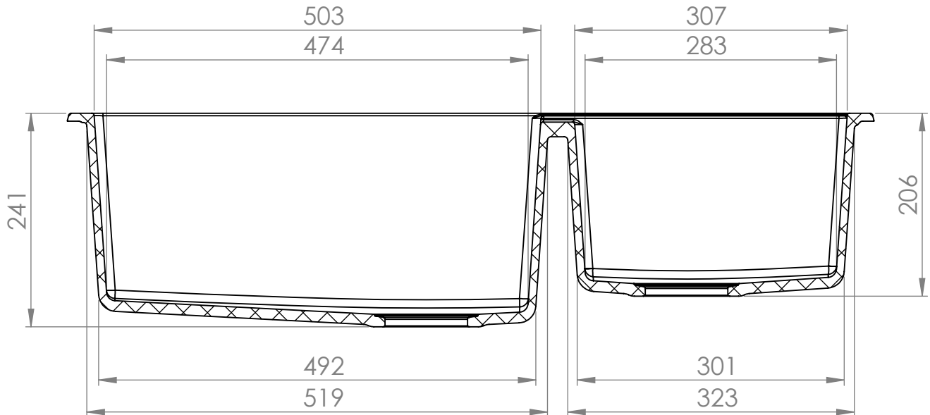
SECTION C-C
